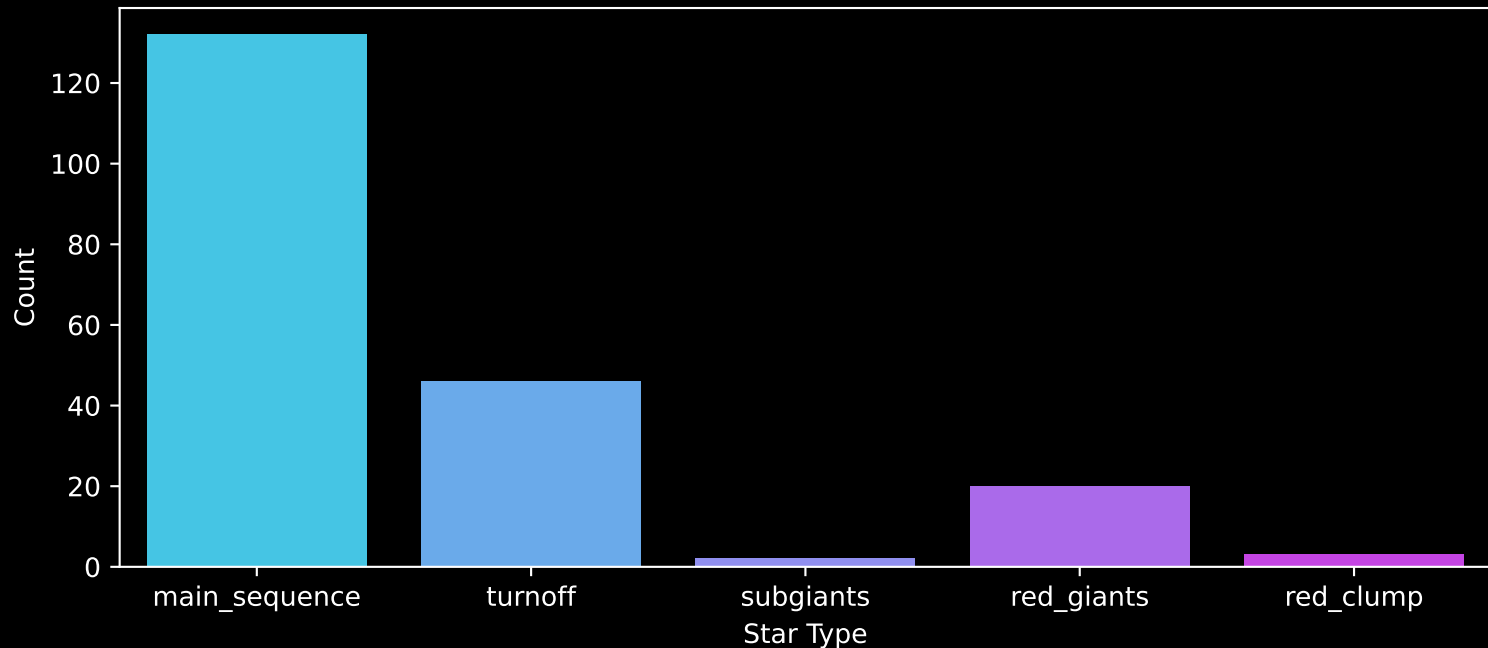
APOGEE DR17 Field: [ALPHAPER] Count plot of Star Type
