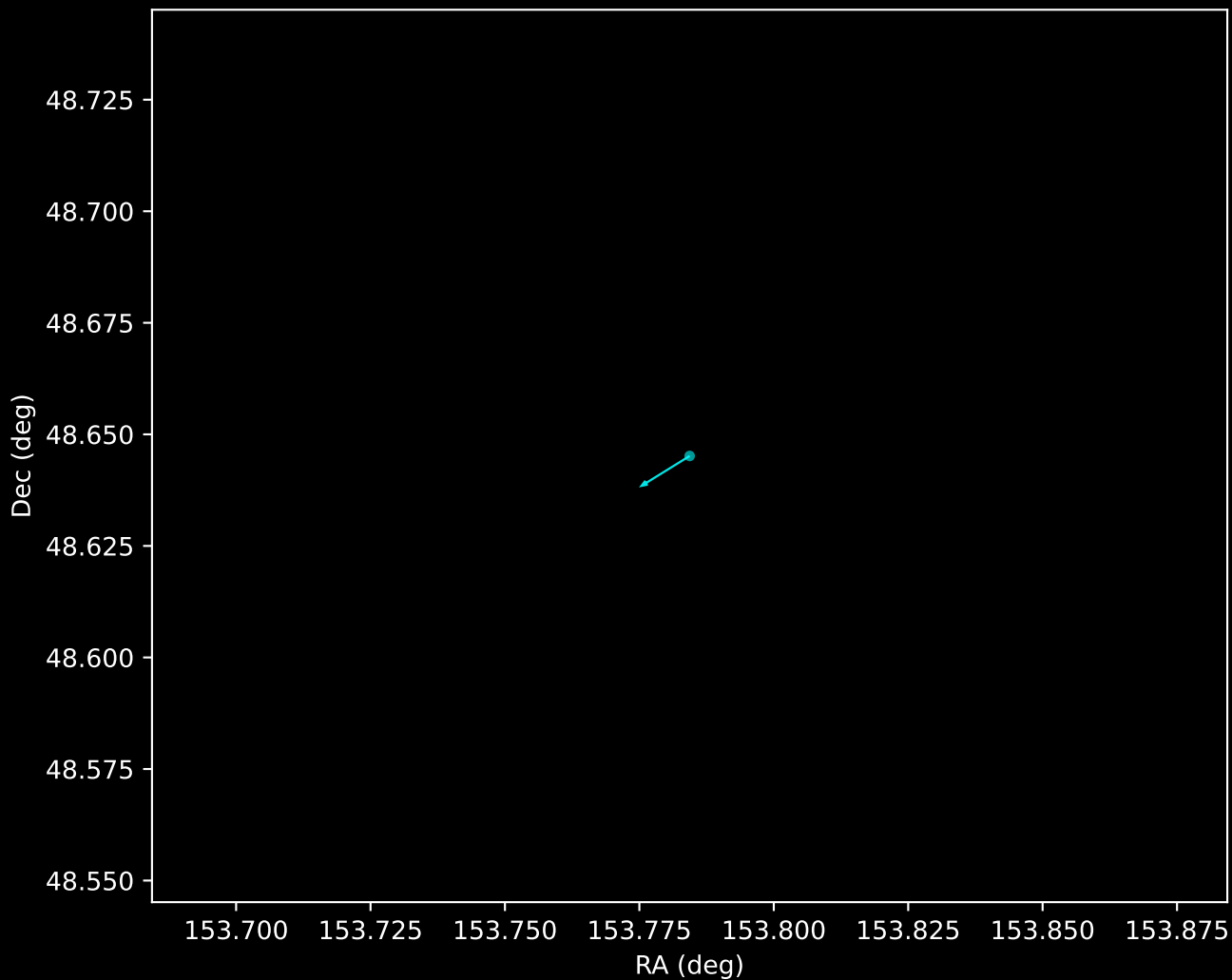
APOGEE DR17 Noise Stream Proper Motion Vectors (n=1)
