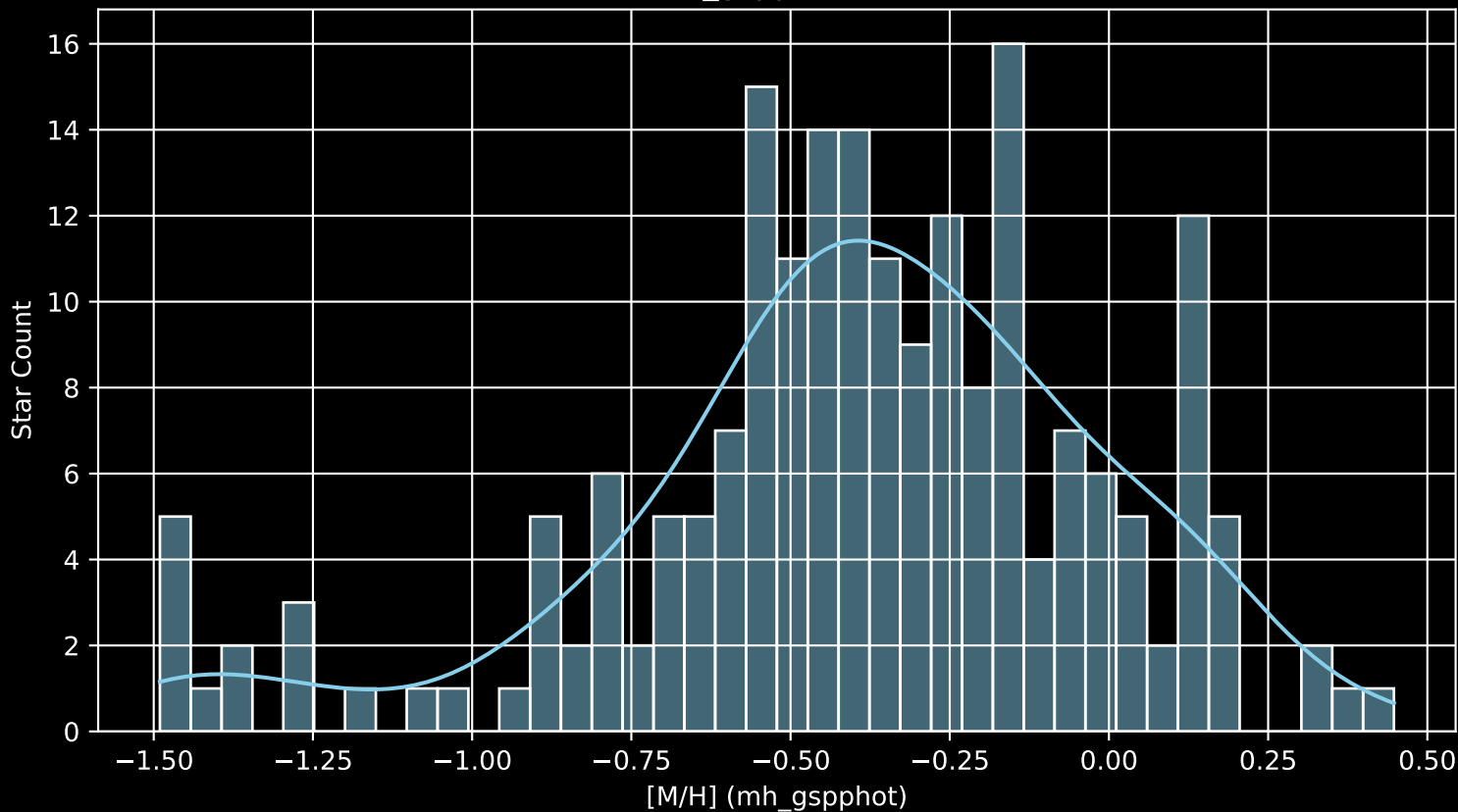
APOGEE DR17 Field: [ALPHAPER [M/H] (mh_gspphot) (n= 202)
