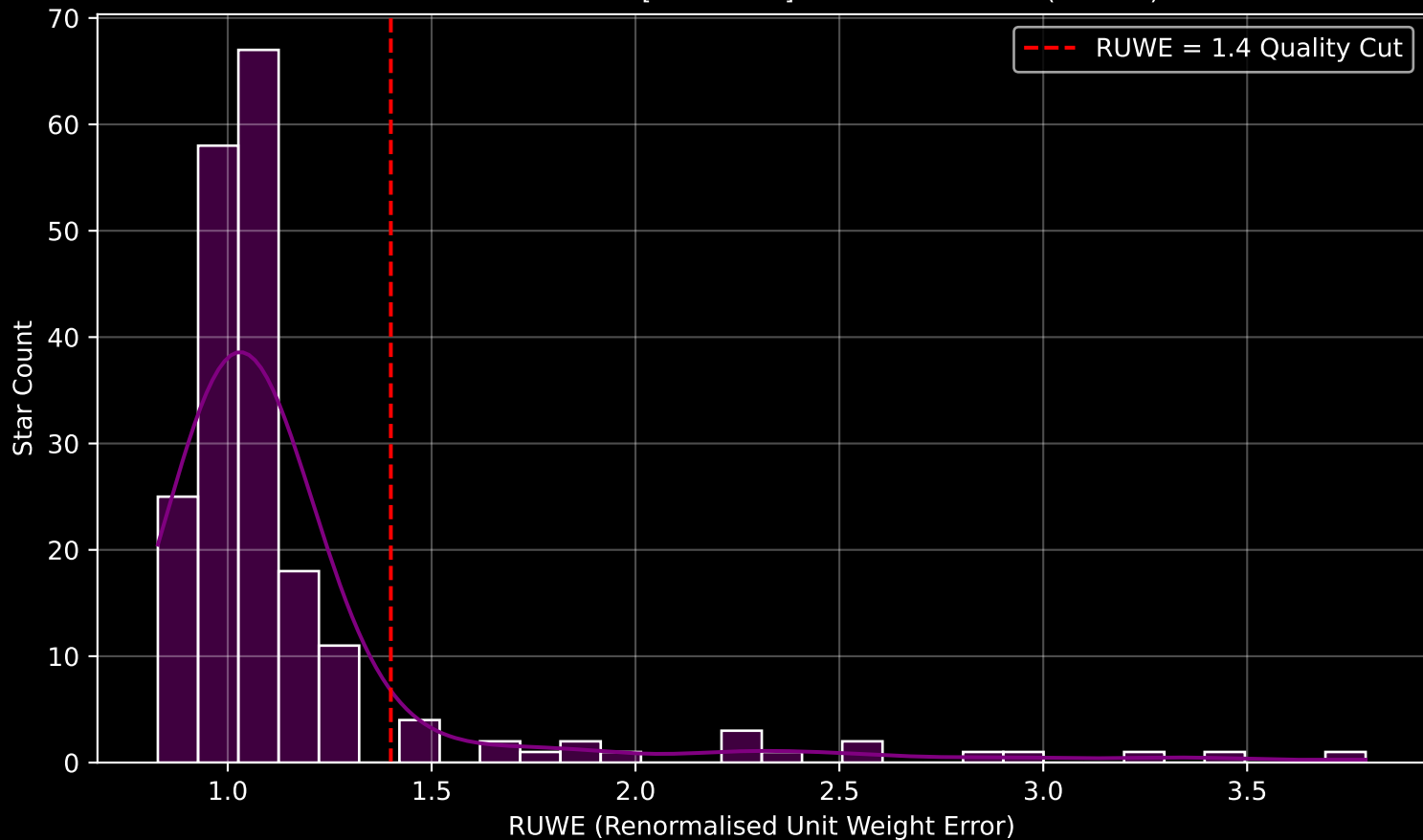
GAPOGEE DR17 Field [ALHPAPER] RUWE Distribution (n= 200)
