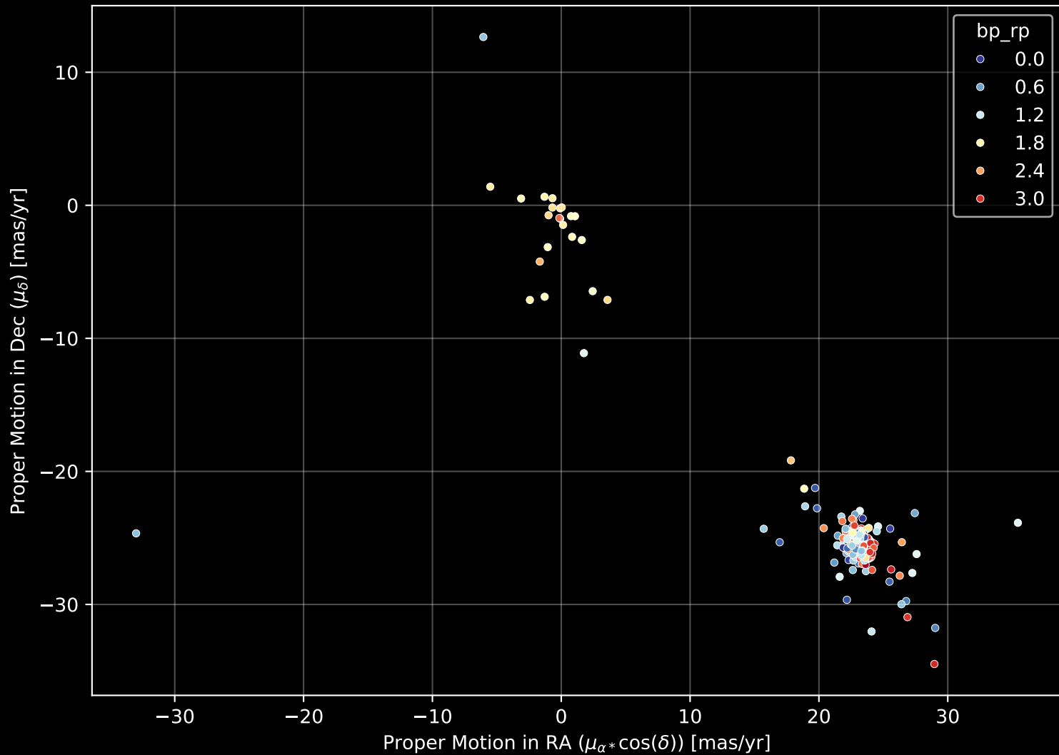
APOGEE DR17 Field: [ALPHAPER] Proper Motion Diagram (n= 203)
