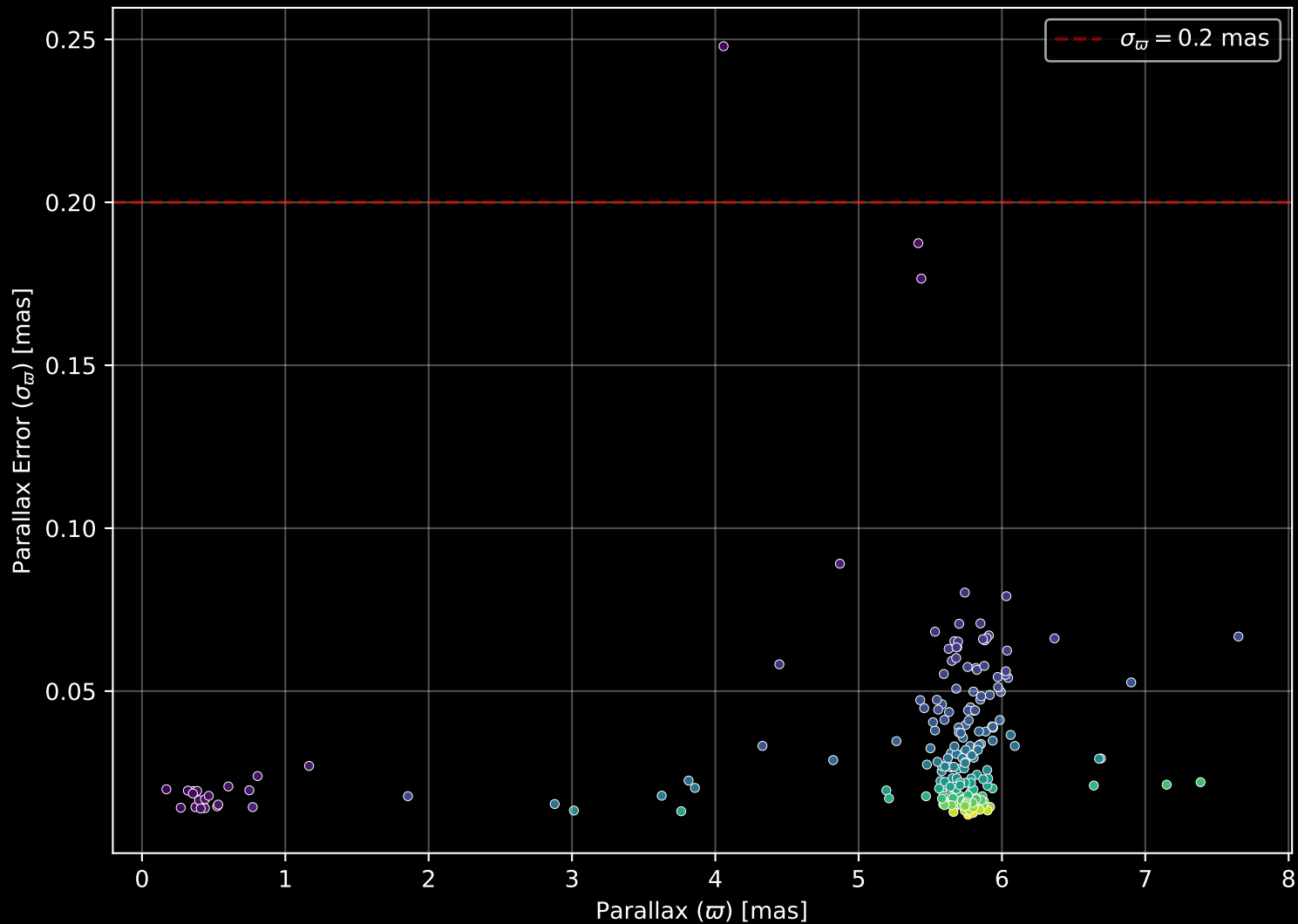
APOGEE DR17 Field: [ALPHAPER] Parallax Quality (n= 203)
